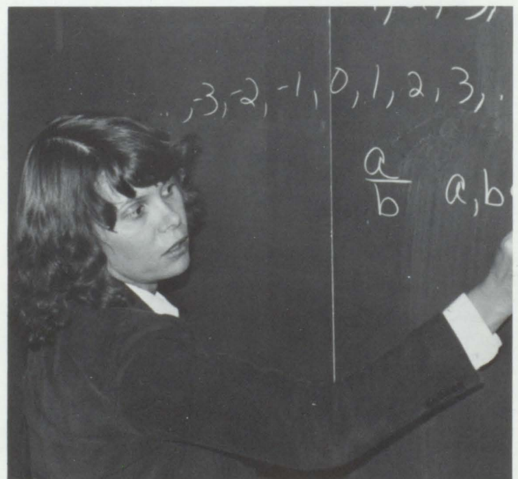
Mrs. Brown gives an explanation for a complex SDL Geometry problem.
