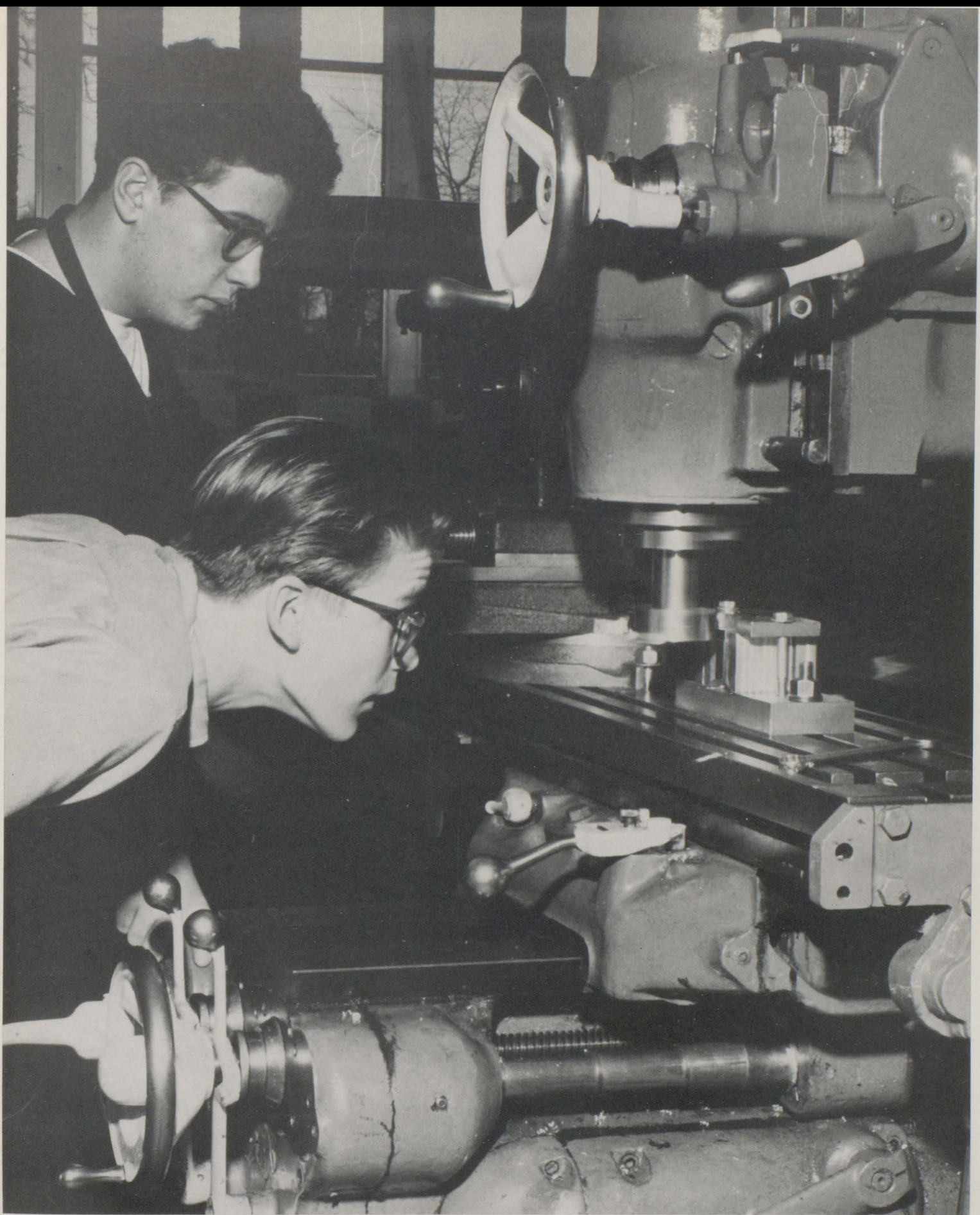
Flycutting the radius on an aluminum meat tenderizer, Craig Cheffer and Tony Bartosz use vertical milling machine.
